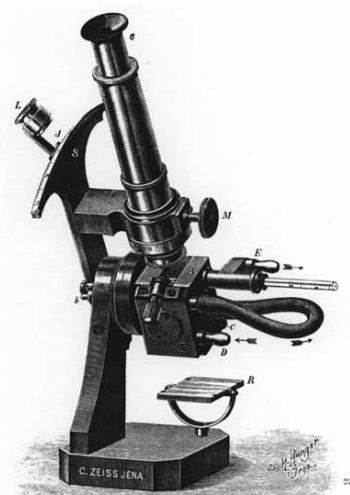
Fig. 1 (1/2 full size). ABBE Refractometer with Heatable Prisms.
